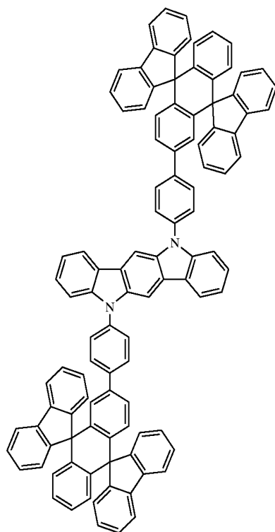
Chemical Compound 409
