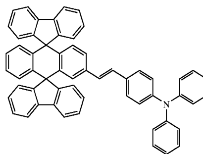
Chemical Compound 400
