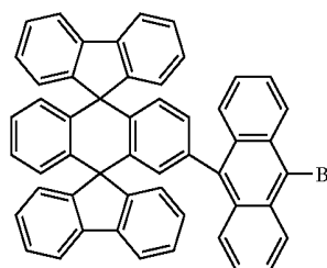
Chemical Compound 5
