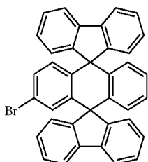
Chemical Compound 1
