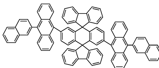
Chemical Compound 115
