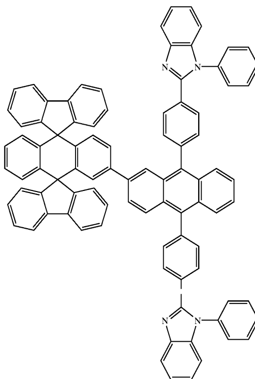
Chemical Compound 206
