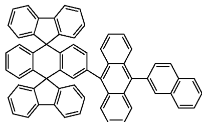
Chemical Compound 110
