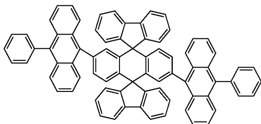
Chemical Compound 114
