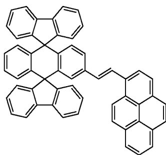
Chemical Compound 103
