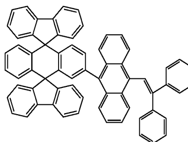
Chemical Compound 137
