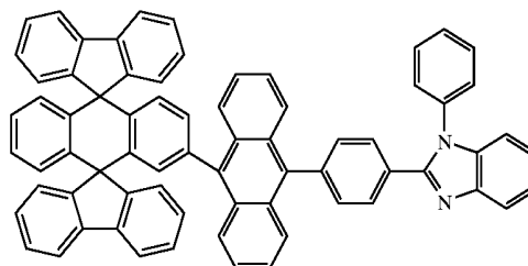
Chemical Compound 204
