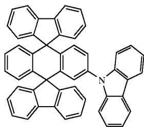
Chemical Compound 404
