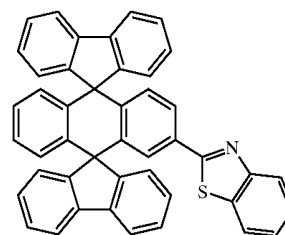
Chemical Compound 215
