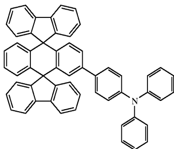
Chemical Compound 303
