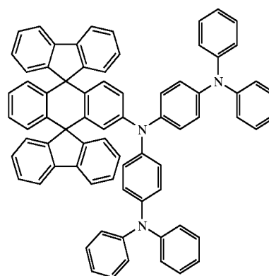
Chemical Compound 308
