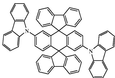
Chemical Compound 407
