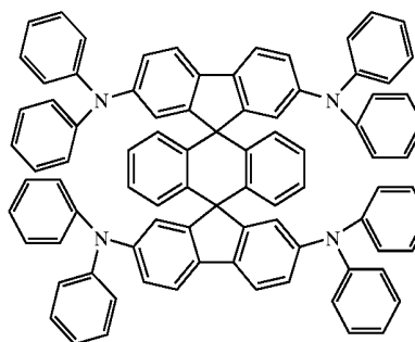
Chemical Compound 304
