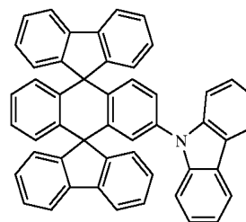
Chemical Compound 10
