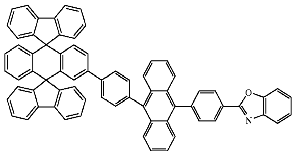
Chemical Compound 126
