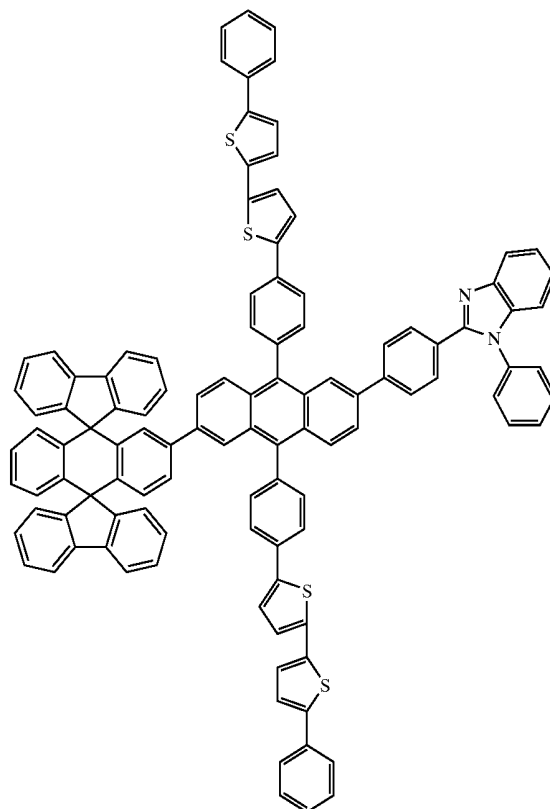
Chemical Compound 130
