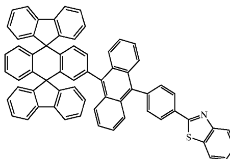
Chemical Compound 217
