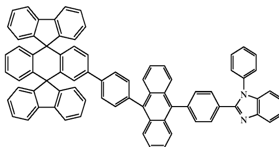
Chemical Compound 210
