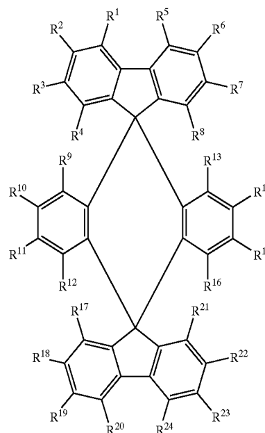
Chemical Formula 1
