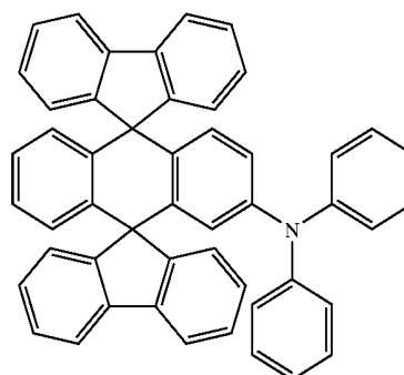
Chemical Compound 300
