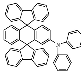
Chemical Compound 11
