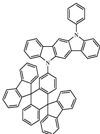
Chemical Compound 410
