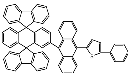
Chemical Compound 134
