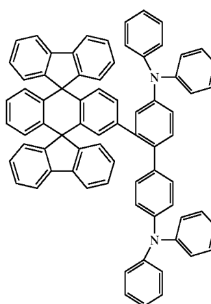
Chemical Compound 305
