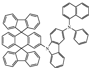
Chemical Compound 306
