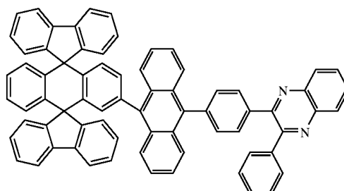
Chemical Compound 209
