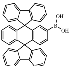
Chemical Compound 8
