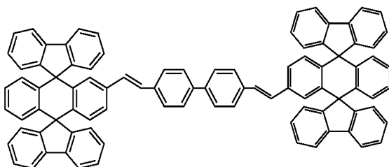
Chemical Compound 100
