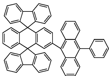
Chemical Compound 109
