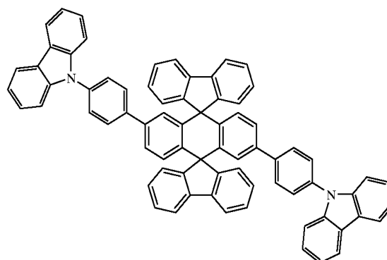
Chemical Compound 402
