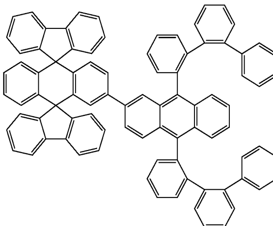
Chemical Compound 136
