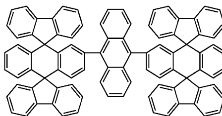
Chemical Compound 102
