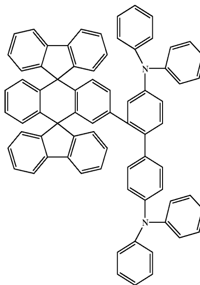
Chemical Compound 305
