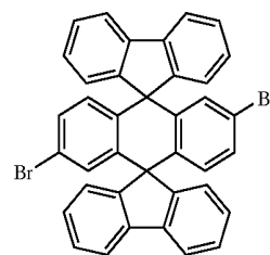
Chemical Compound 2
