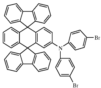
Chemical Compound 7
