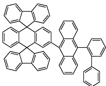
Chemical Compound 111
