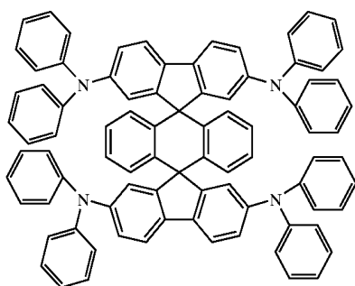
Chemical Compound 304
