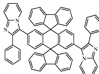
Chemical Compound 413.
