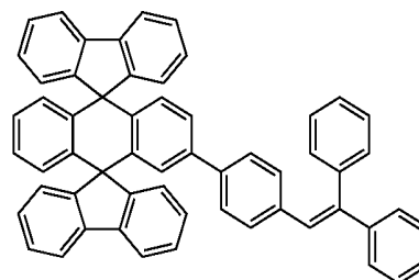
Chemical Compound 107
