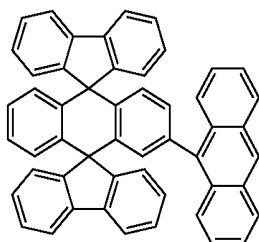
Chemical Compound 9
