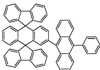
Chemical Compound 109
