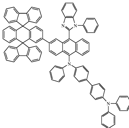
Chemical Compound 125
