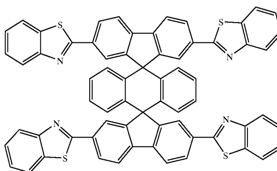
Chemical Compound 218
