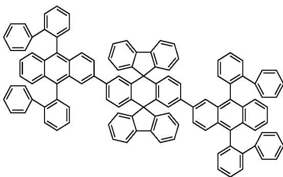
Chemical Compound 121
