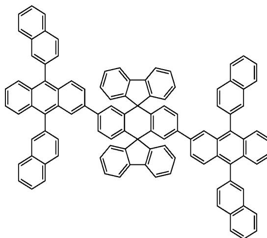
Chemical Compound 123
