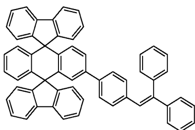
Chemical Compound 107
