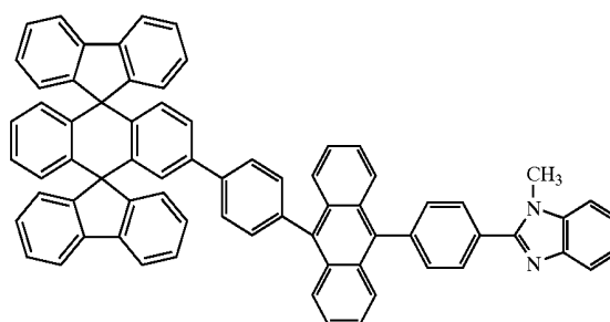
Chemical Compound 211
