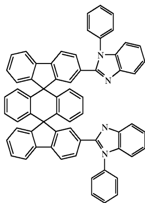
Chemical Compound 221
