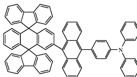
Chemical Compound 401
