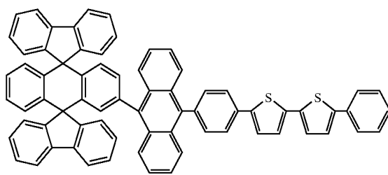
Chemical Compound 131
