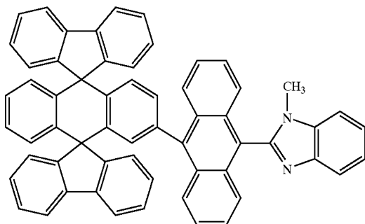
Chemical Compound 205
