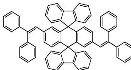
Chemical Compound 105
