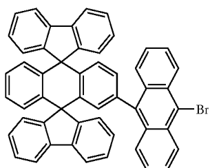
Chemical Compound 5
