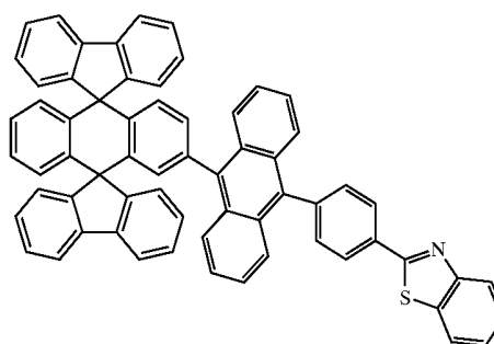
Chemical Compound 217
