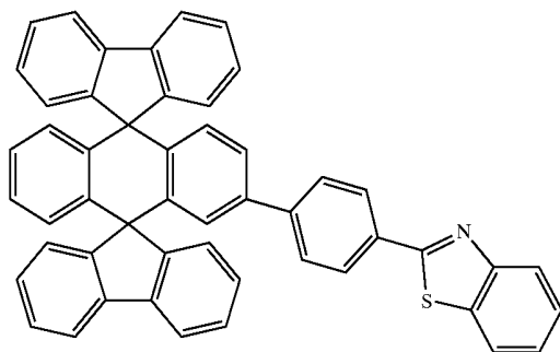
Chemical Compound 213
