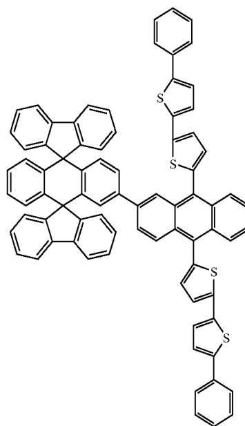
Chemical Compound 128
