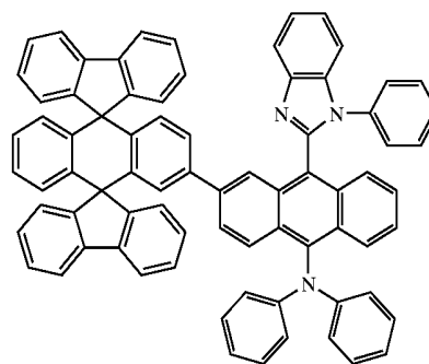
Chemical Compound 127
