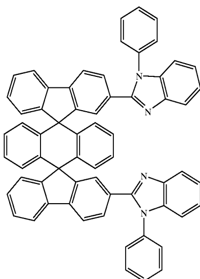
Chemical Compound 221
