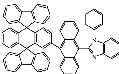
Chemical Compound 200
