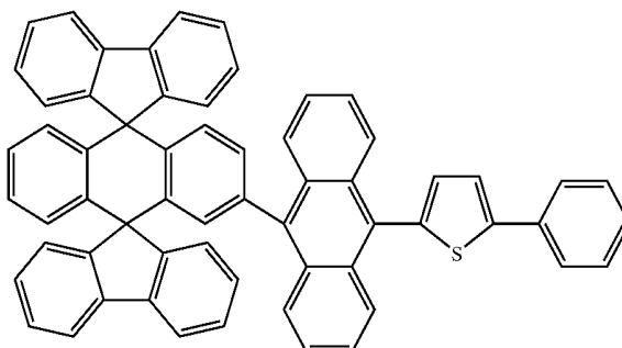
Chemical Compound 134
