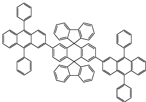
Chemical Compound 122
