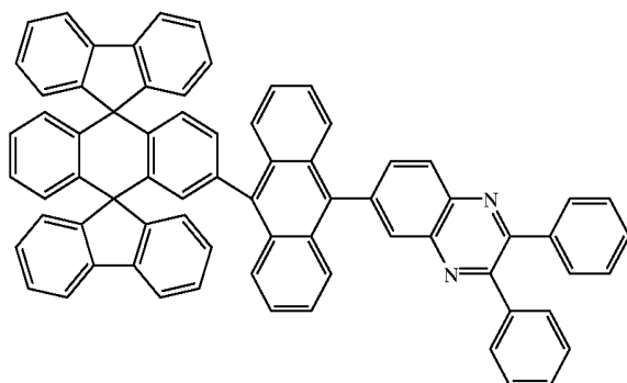
Chemical Compound 203
