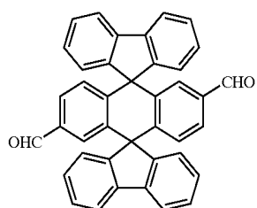
Chemical Compound 4
