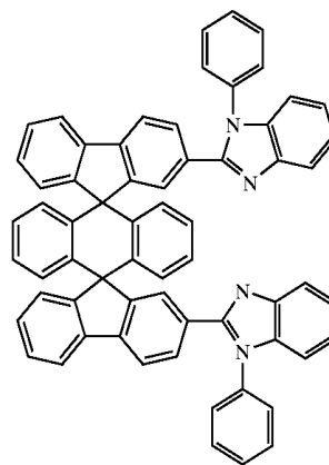
Chemical Compound 221
