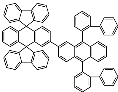
Chemical Compound 118
