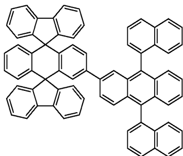
Chemical Compound 120
