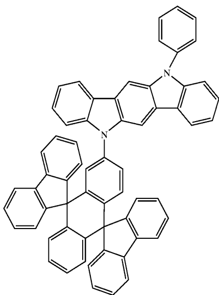
Chemical Compound 410
