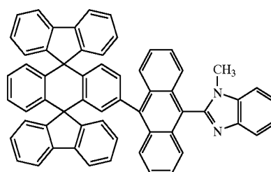
Chemical Compound 205
