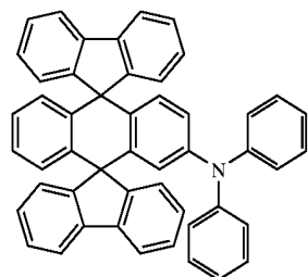
Chemical Compound 300
