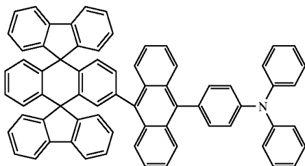
Chemical Compound 400
