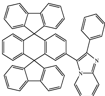
Chemical Compound 412
