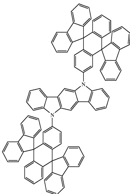
Chemical Compound 405
