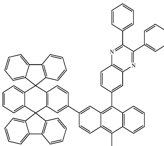
Chemical Compound 212
