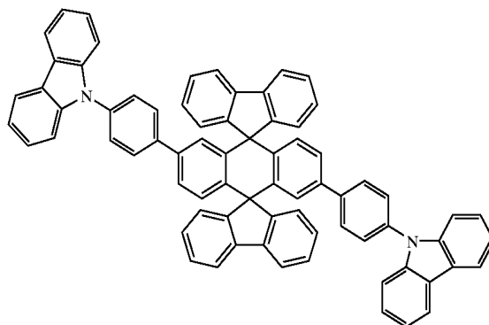
Chemical Compound 402
