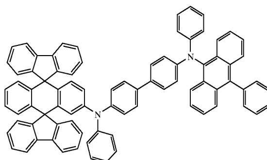
Chemical Compound 408
