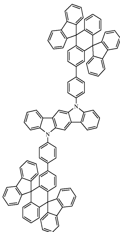
Chemical Compound 409
