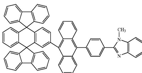
Chemical Compound 208
