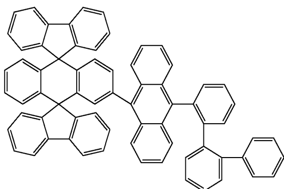
Chemical Compound 112
