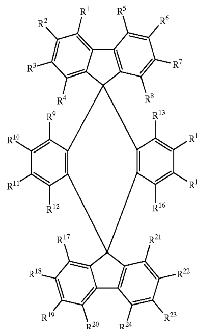
Chemical Formula 1
