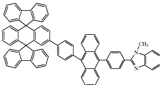
Chemical Compound 211
