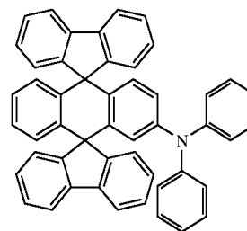
Chemical Compound 300
