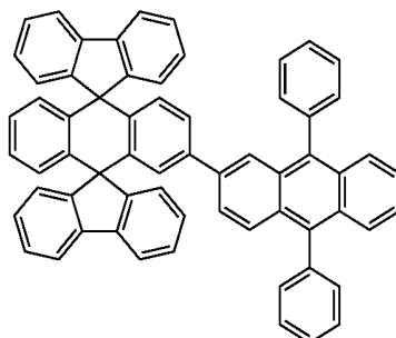
Chemical Compound 116
