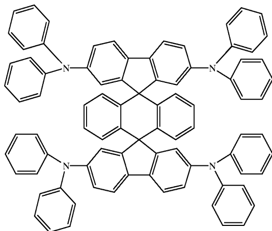
Chemical Compound 304
