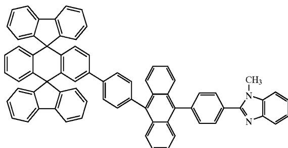
Chemical Compound 211
