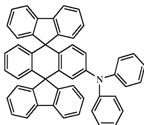
Chemical Compound 11
