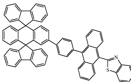
Chemical Compound 216
