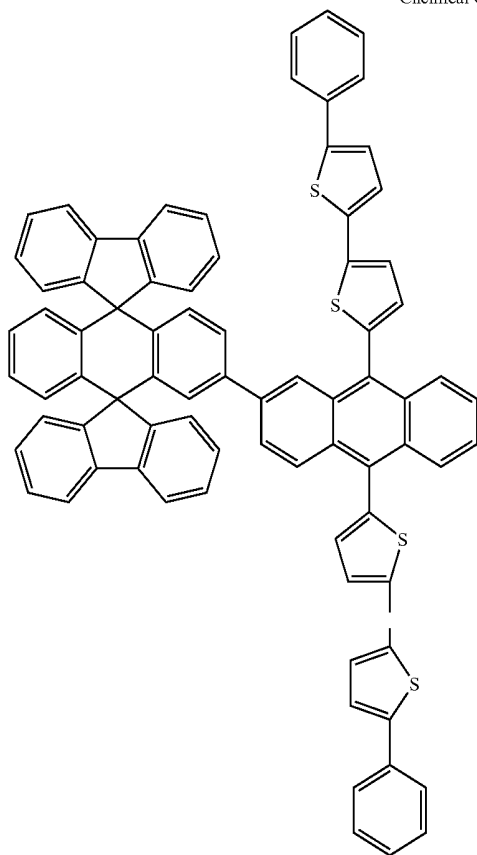
Chemical Compound 128
