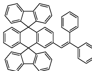
Chemical Compound 106
