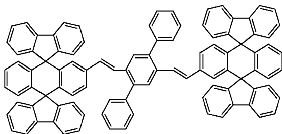
Chemical Compound 101
