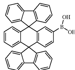
Chemical Compound 8
