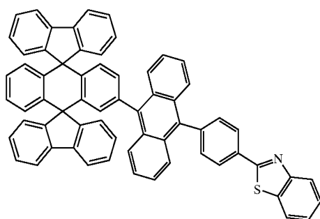
Chemical Compound 217
