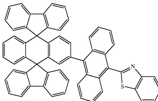
Chemical Compound 214
