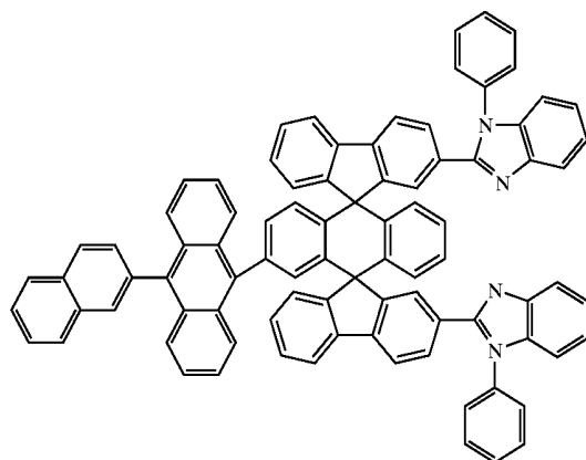
Chemical Compound 222
