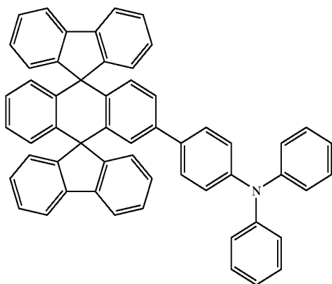
Chemical Compound 303
