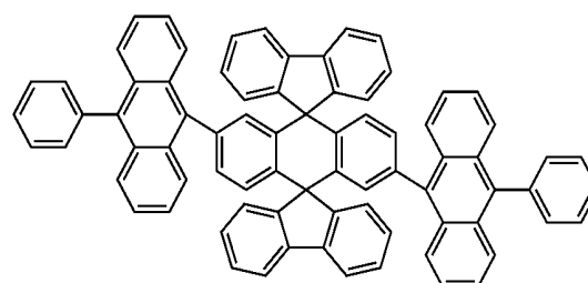
Chemical Compound 114
