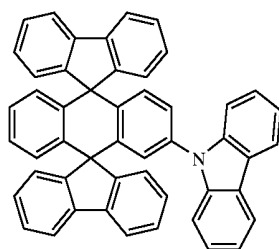
Chemical Compound 10
