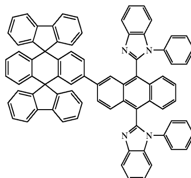
Chemical Compound 202
