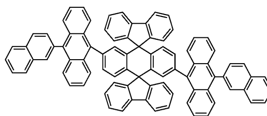
Chemical Compound 115
