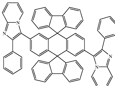
Chemical Compound 413
