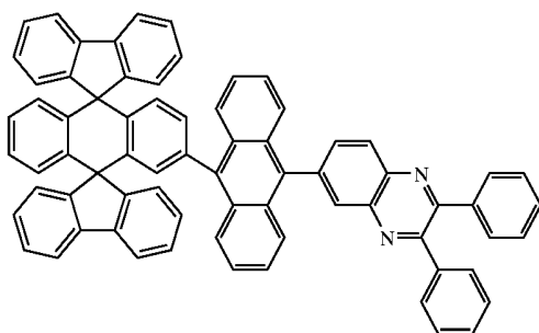
Chemical Compound 203
