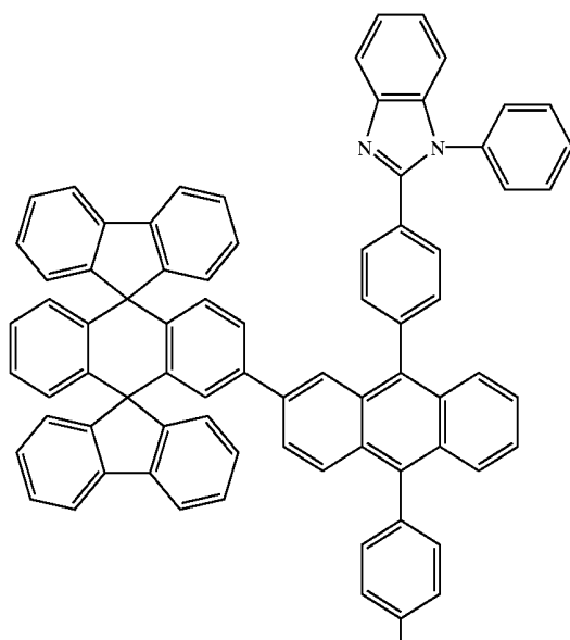
Chemical Compound 206
