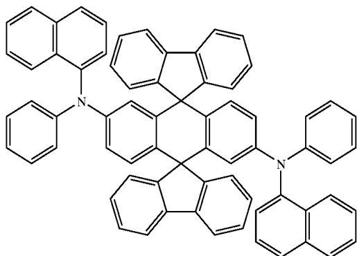
Chemical Compound 302
