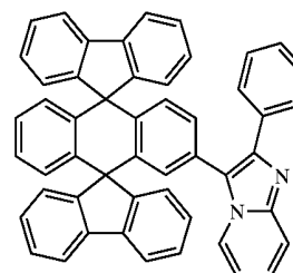
Chemical compound 412
