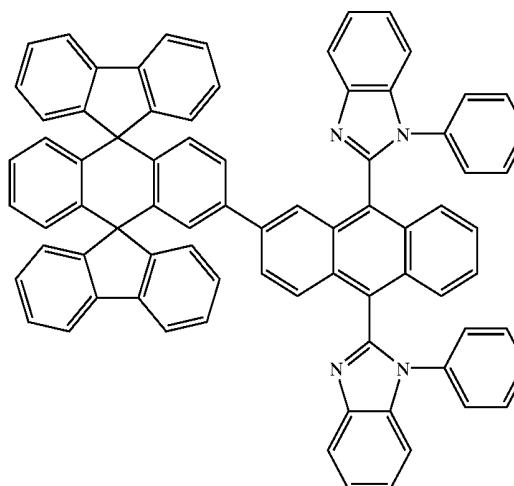
Chemical Compound 202
