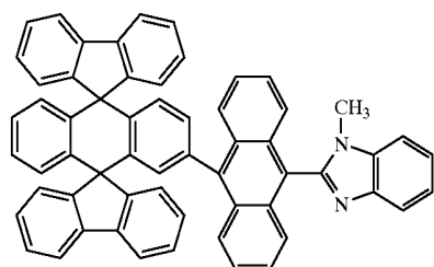
Chemical Compound 205
