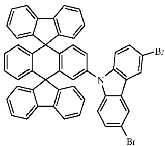
Chemical Compound 6
