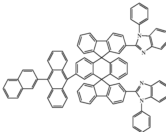
Chemical Compound 222
