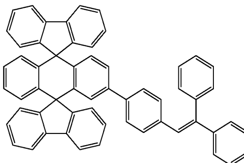
Chemical Compound 107
