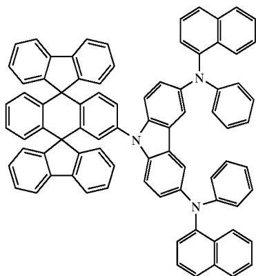
Chemical Compound 403
