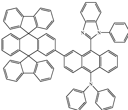
Chemical Compound 127
