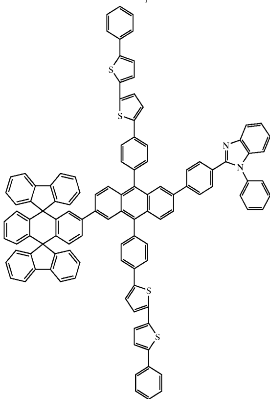
Chemical Compound 130
