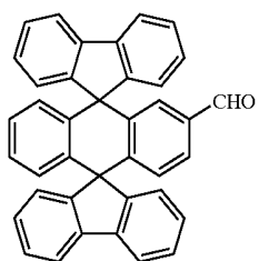
Chemical Compound 3
