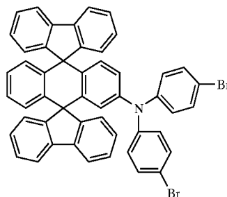
Chemical Compound 7
