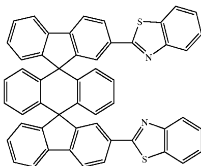
Chemical Compound 220
