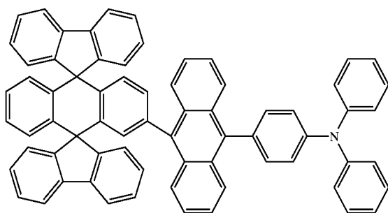
Chemical Compound 401
