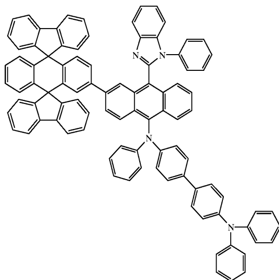
Chemical Compound 125
