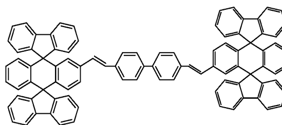
Chemical Compound 100
