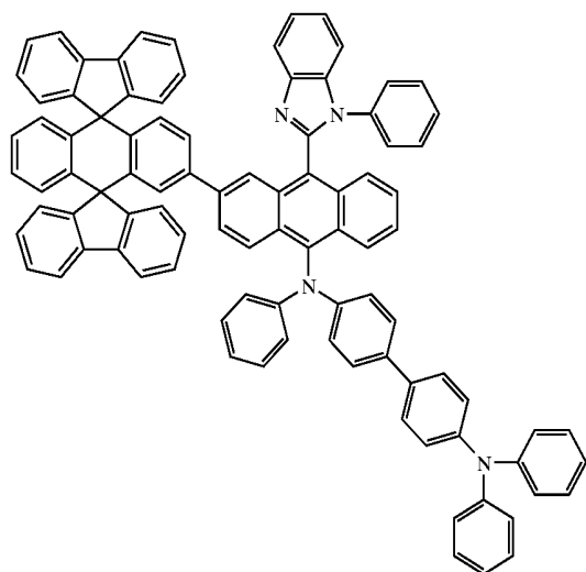
Chemical Compound 125
