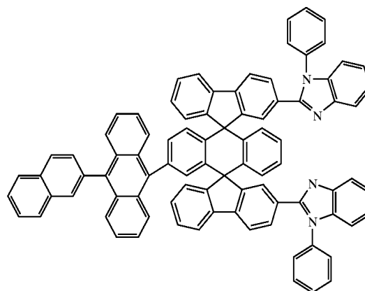
Chemical Compound 222
