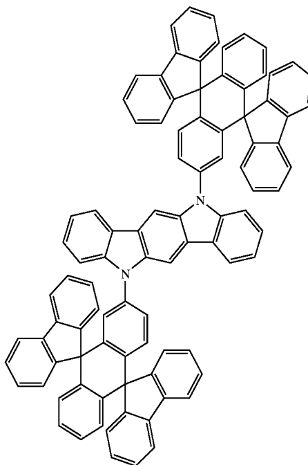
Chemical Compound 405
