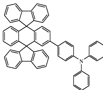
Chemical Compound 303
