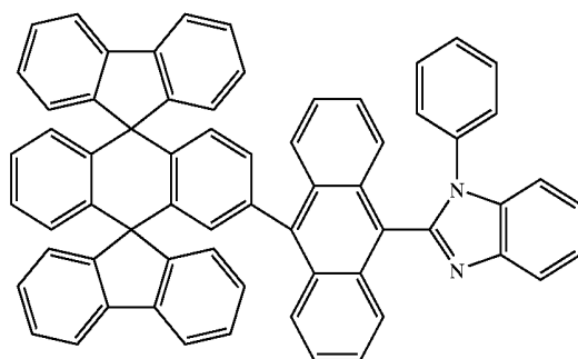
Chemical Compound 201
