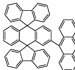
Chemical Compound 9
