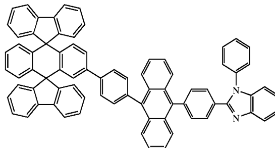
Chemical Compound 210
