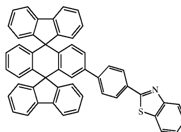
Chemical Compound 213
