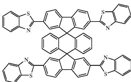
Chemical Compound 218
