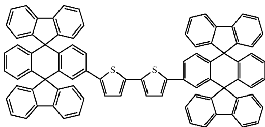
Chemical Compound 135
