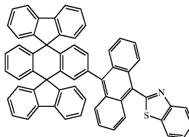
Chemical Compound 214
