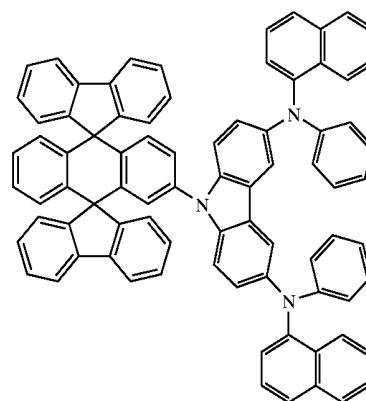
Chemical Compound 403
