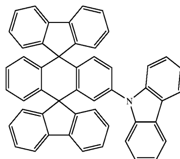
Chemical Compound 404
