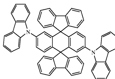
Chemical Compound 407
