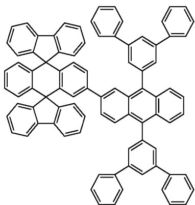
Chemical Compound 119
