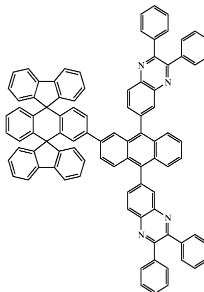
Chemical Compound 212
