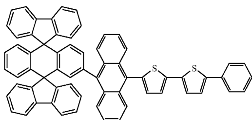
Chemical Compound 133
