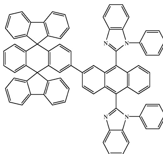
Chemical Compound 203
