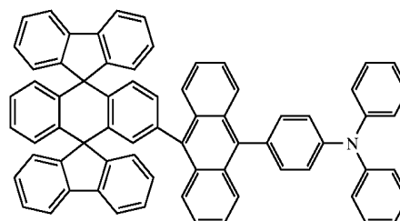
Chemical Compound 401
