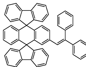
Chemical Compound 106
