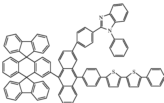
Chemical Compound 132
