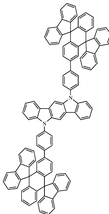
Chemical Compound 409
