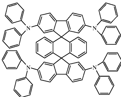
Chemical Compound 304
