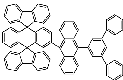
Chemical Compound 113
