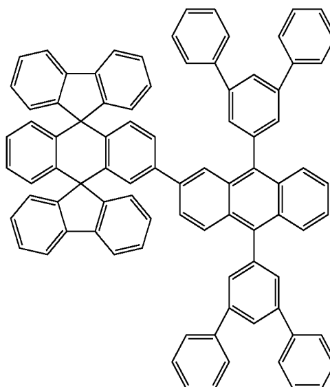
Chemical Compound 119
