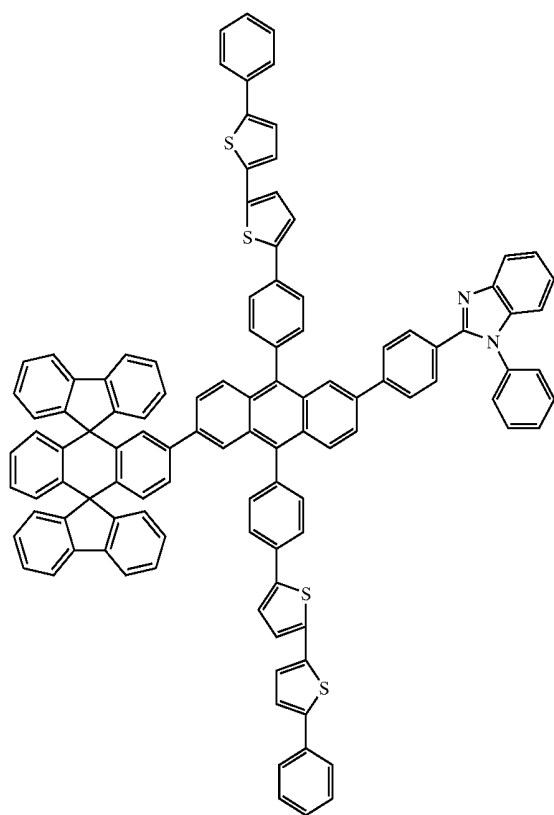
Chemical Compound 130
