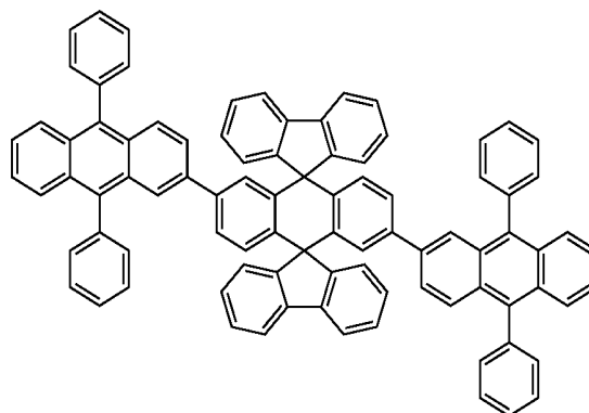
Chemical Compound 122
