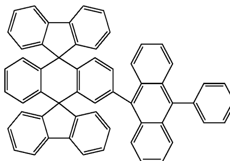
Chemical Compound 109
