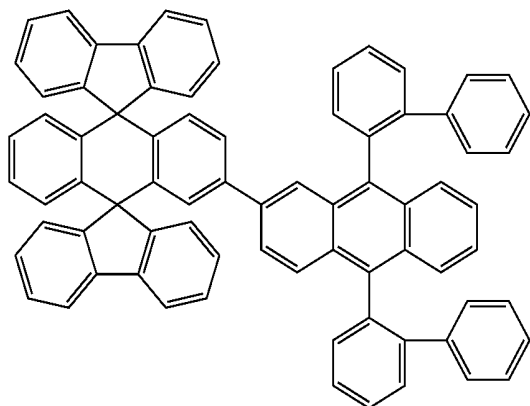
Chemical Compound 118
