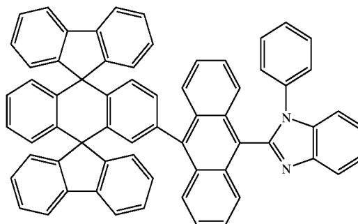
Chemical Compound 200
