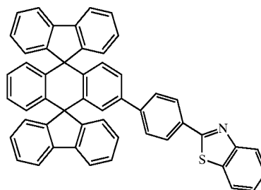
Chemical Compound 213
