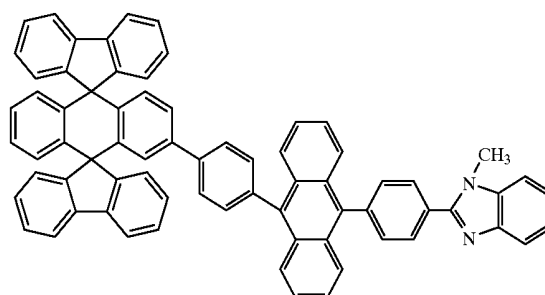
Chemical Compound 211
