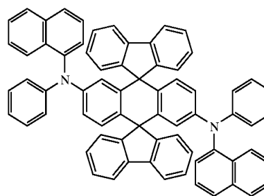
Chemical Compound 302
