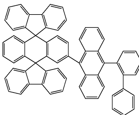
Chemical Compound 111
