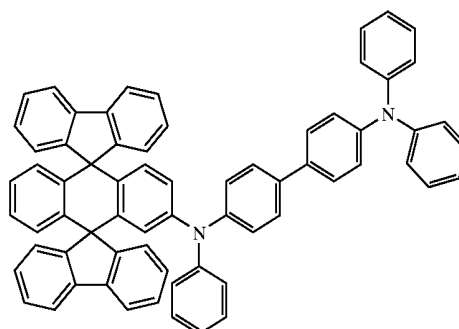
Chemical Compound 307
