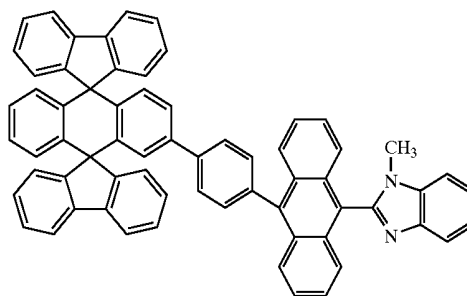
Chemical Compound 201
