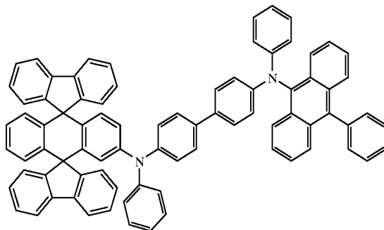
Chemical Compound 408
