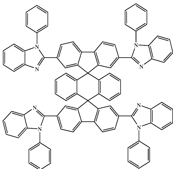
Chemical Compound 219
