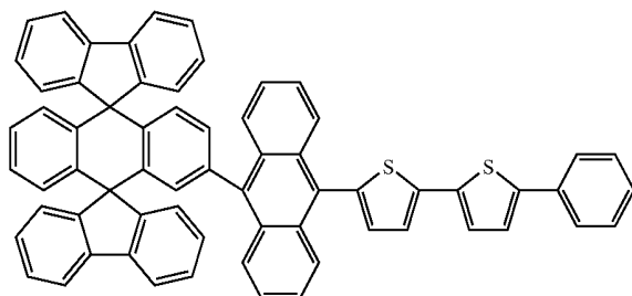
Chemical Compound 133
