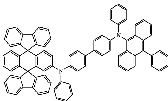
Chemical Compound 408
