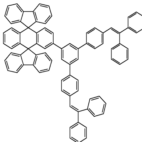
Chemical Compound 108
