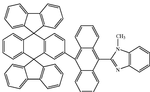
Chemical Compound 205
