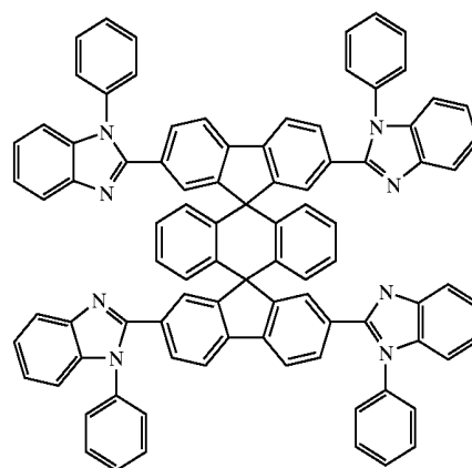
Chemical Compound 219
