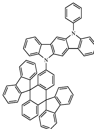
Chemical Compound 410
