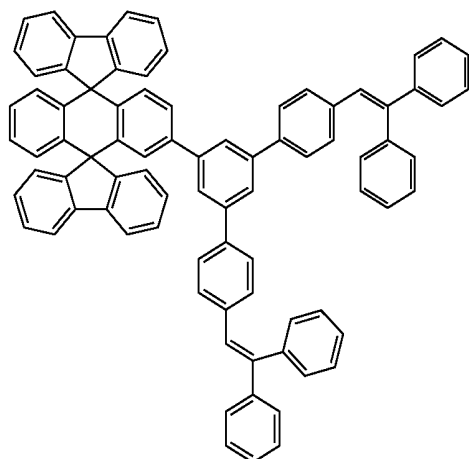
Chemical Compound 108
