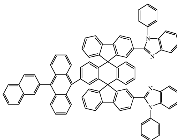
Chemical Compound 222
