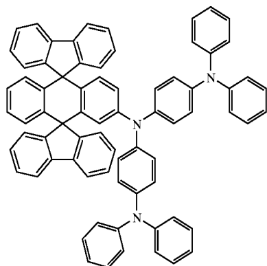
Chemical Compound 308
