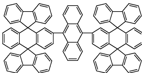
Chemical Compound 102
