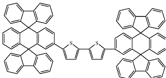
Chemical Compound 135
