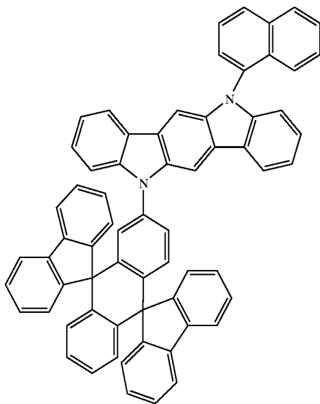
Chemical Compound 412
