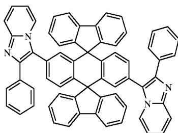
Chemical Compound 413.
