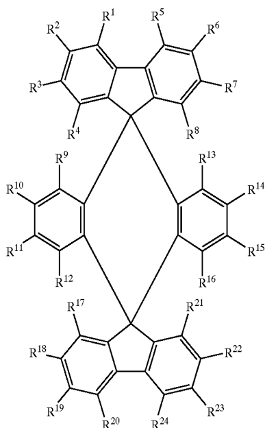
Chemical Formula 1
