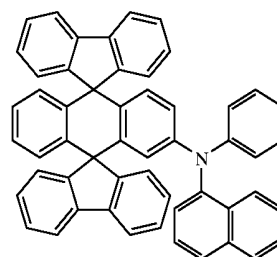
Chemical Compound 301
