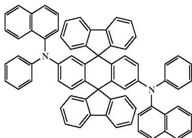
Chemical Compound 302
