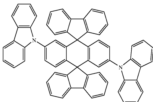
Chemical Compound 407
