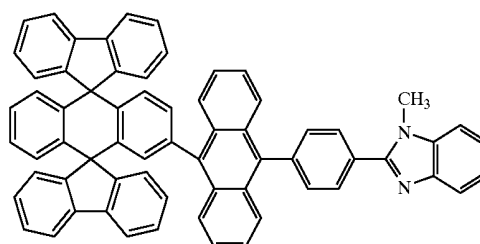
Chemical Compound 208
