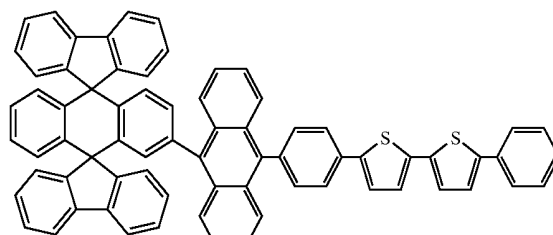
Chemical Compound 131
