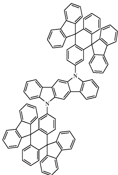
Chemical Compound 405
