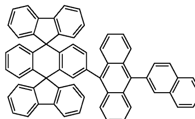
Chemical Compound 110
