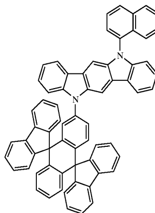
Chemical Compound 411
