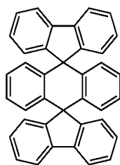
Chemical Compound 12
