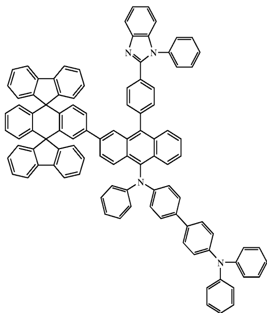
Chemical Compound 124
