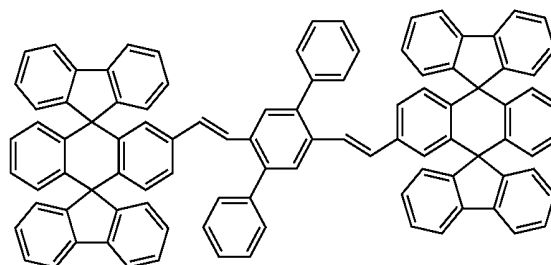
Chemical Compound 101
