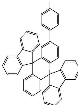
Chemical Compound 407
