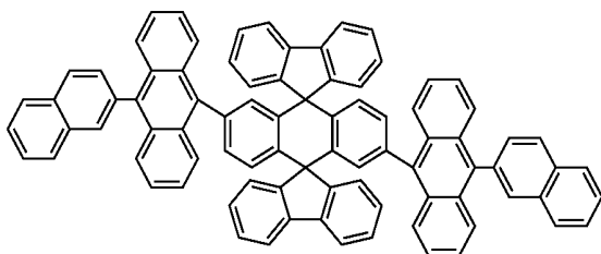
Chemical Compound 115
