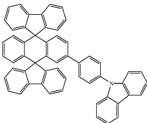
Chemical Compound 406
