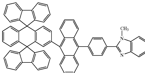
Chemical Compound 208
