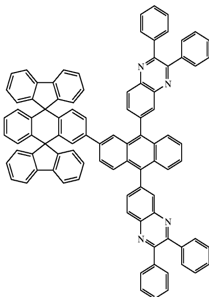
Chemical Compound 212
