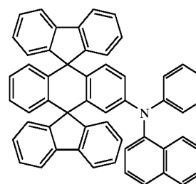
Chemical Compound 301
