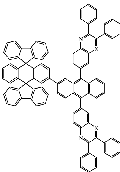
Chemical Compound 212
