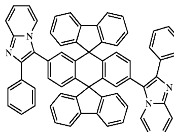
Chemical Compound 413
