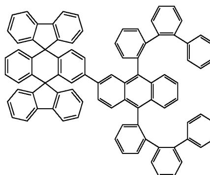
Chemical Compound 136
