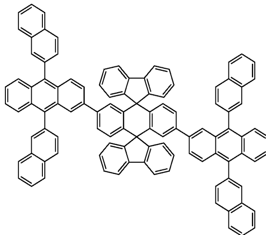
Chemical Compound 123
