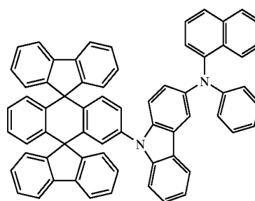
Chemical Compound 306
