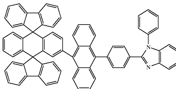
Chemical Compound 204
