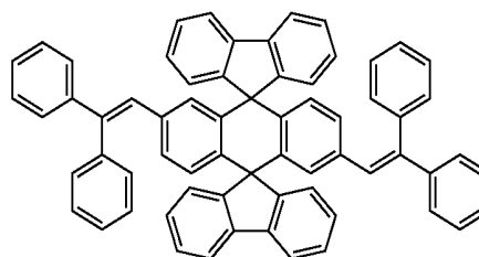
Chemical Compound 105
