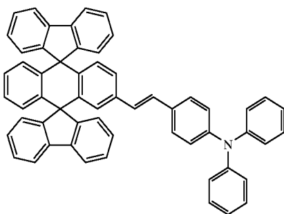
Chemical Compound 400
