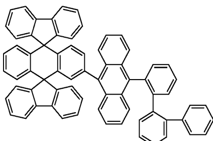
Chemical Compound 112
