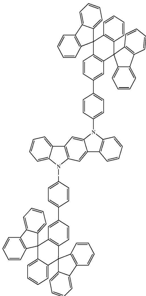
Chemical Compound 409
