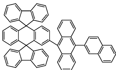
Chemical Compound 110
