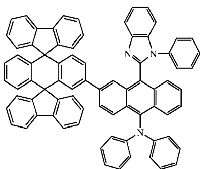
Chemical Compound 127
