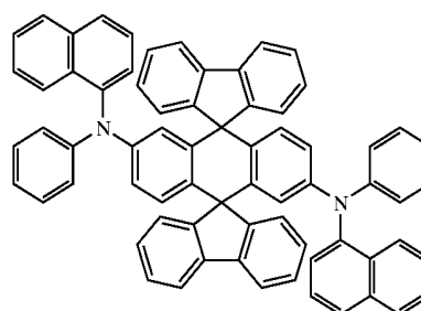
Chemical Compound 302
