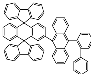
Chemical Compound 111
