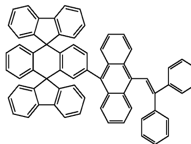
Chemical Compound 137
