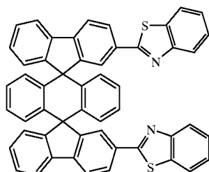
Chemical Compound 220
