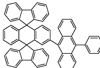
Chemical Compound 109
