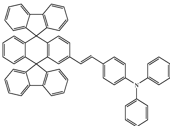
Chemical Compound 400
