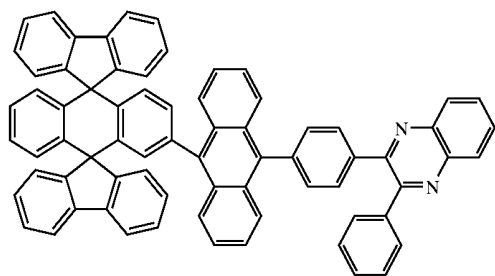
Chemical Compound 209
