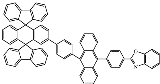
Chemical Compound 126
