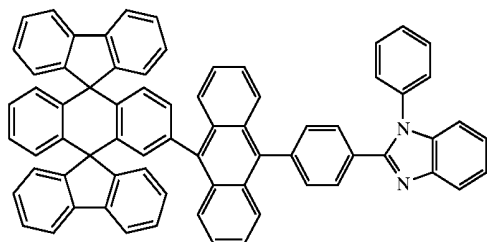
Chemical Compound 204
