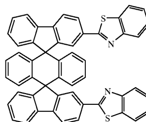
Chemical Compound 220
