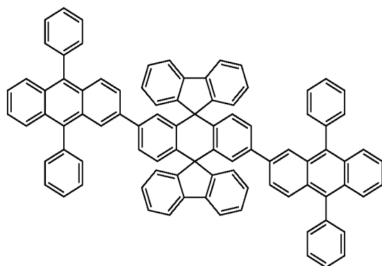
Chemical Compound 122
