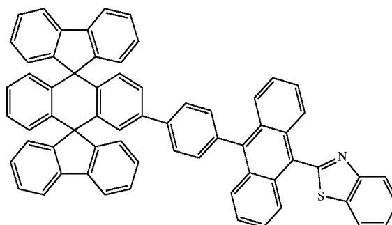
Chemical Compound 216
