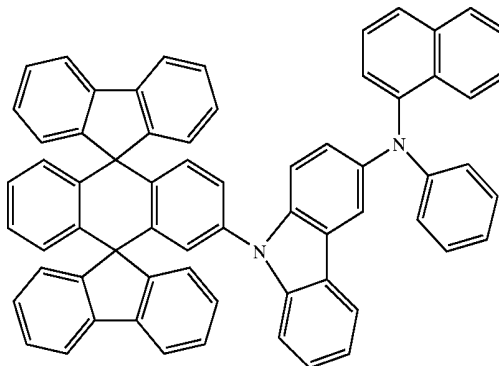
Chemical Compound 306
