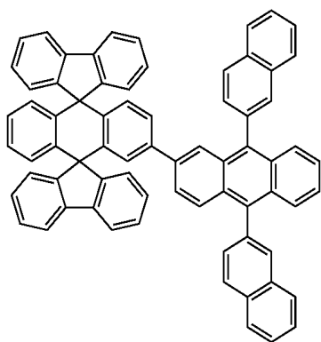
Chemical Compound 117
