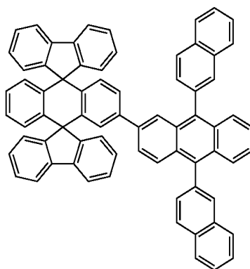
Chemical Compound 117
