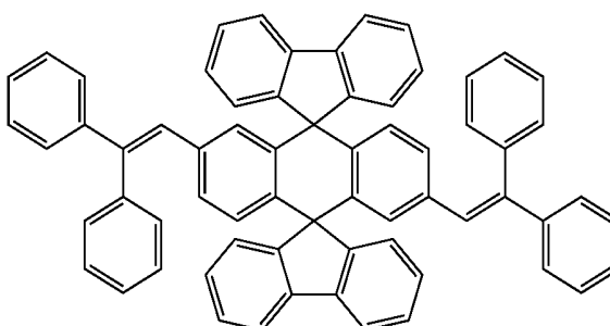
Chemical Compound 105
