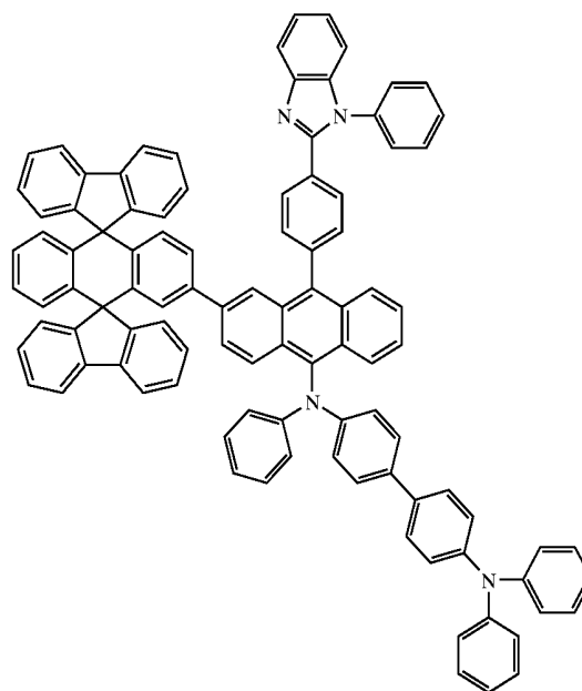
Chemical Compound 124
