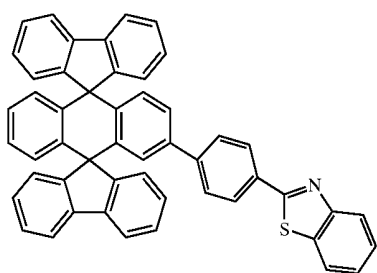
Chemical Compound 213
