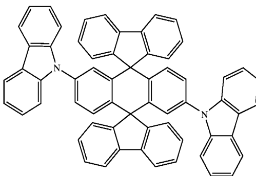
Chemical Compound 407
