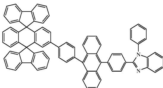
Chemical Compound 210
