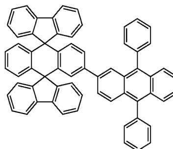
Chemical Compound 116
