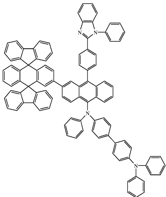
Chemical Compound 124
