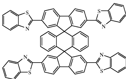
Chemical Compound 218
