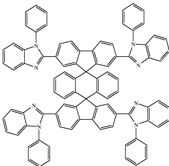
Chemical Compound 219
