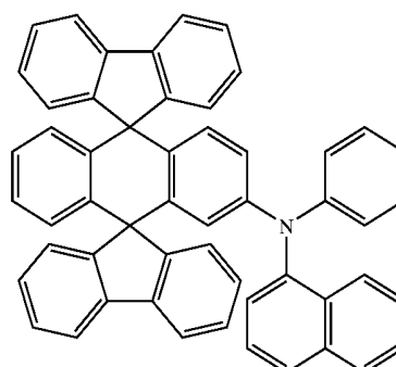
Chemical Compound 301
