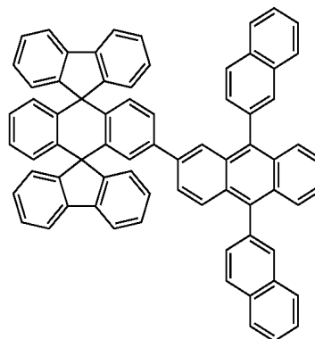
Chemical Compound 117
