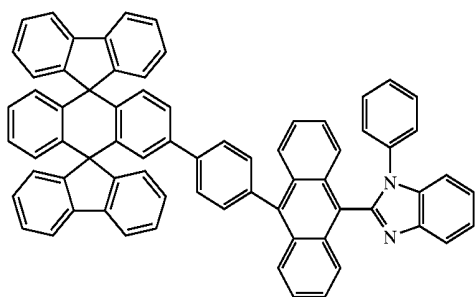
Chemical Compound 207
