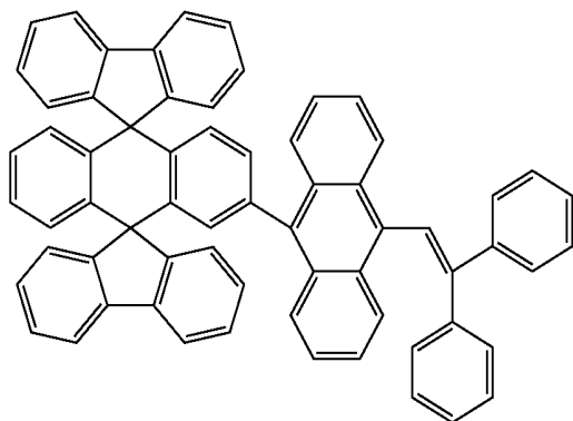
Chemical Compound 137
