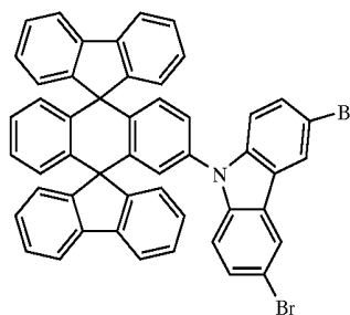
Chemical Compound 6
