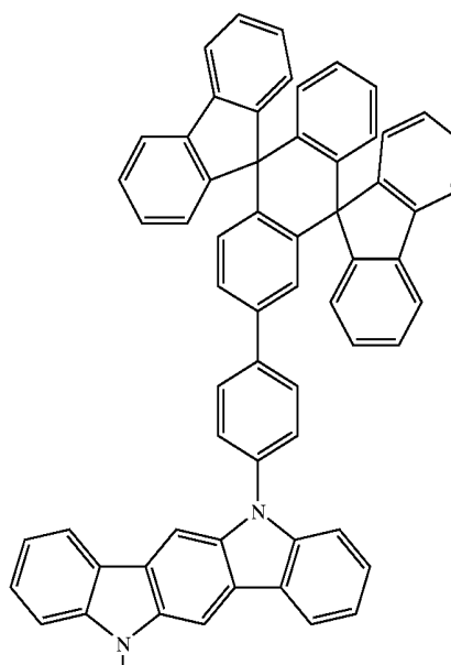
Chemical Compound 409
