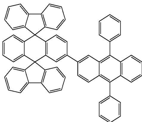
Chemical Compound 116
